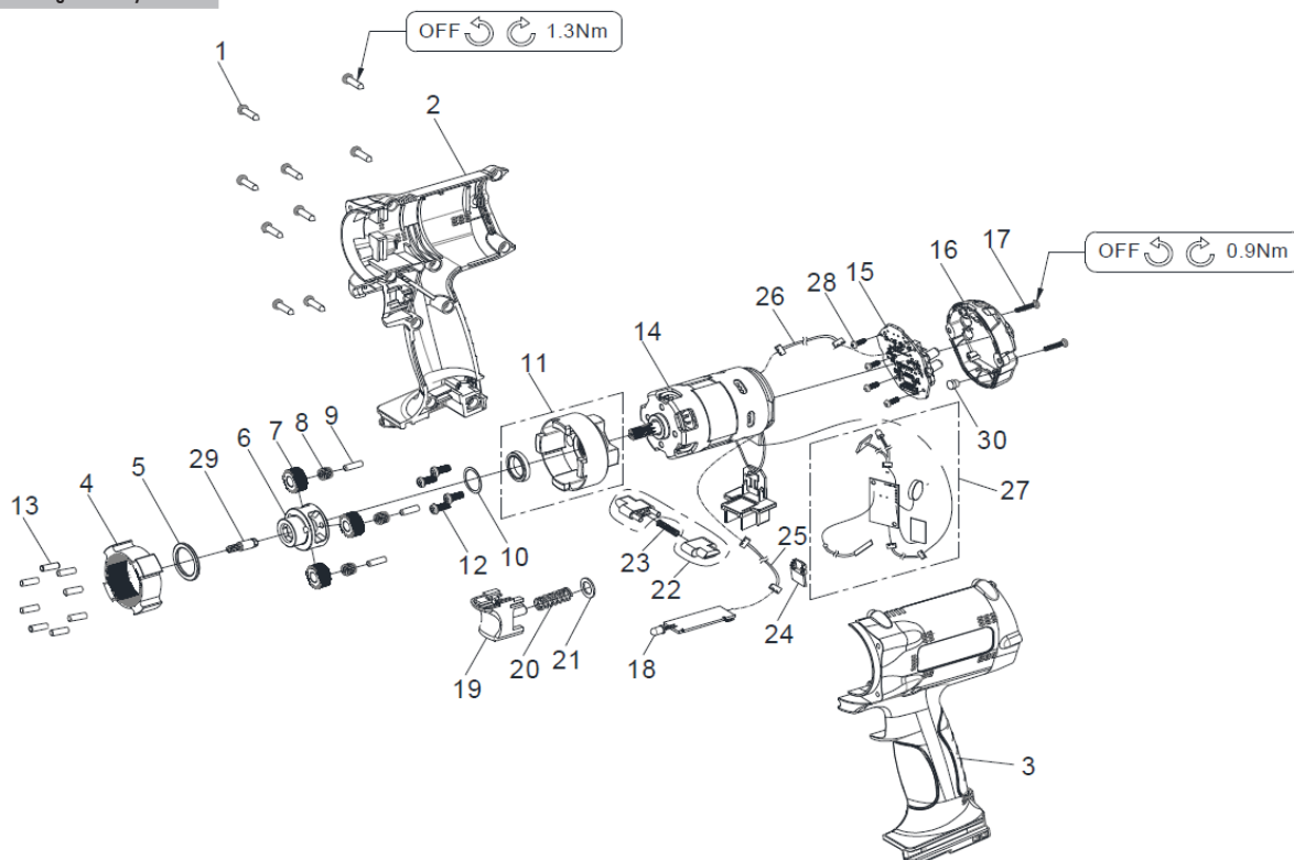
Motor Housing Assembly
