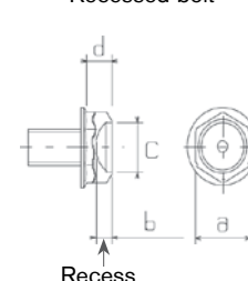
Recessed bolt
