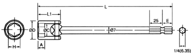
SCREWDRIVER BIT
