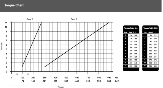
Torque chart (sample)
