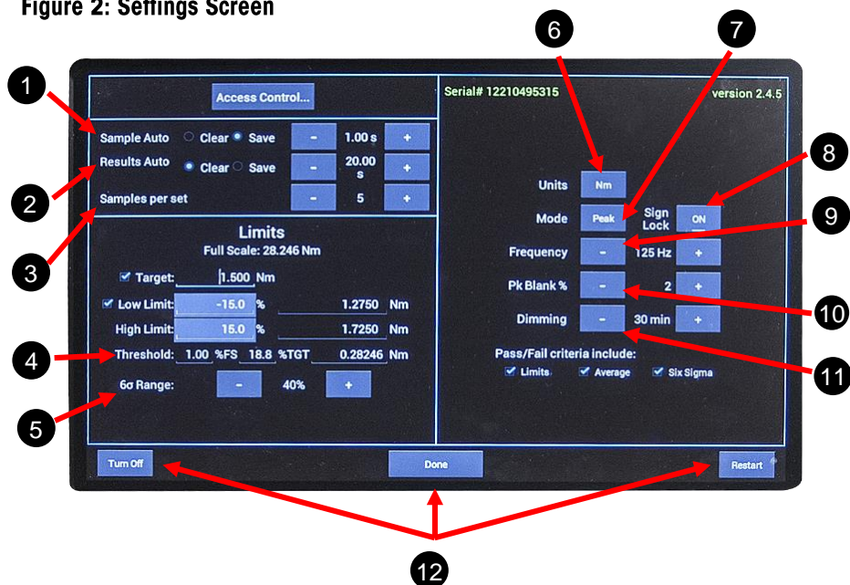
Figure 2: Settings Screen
