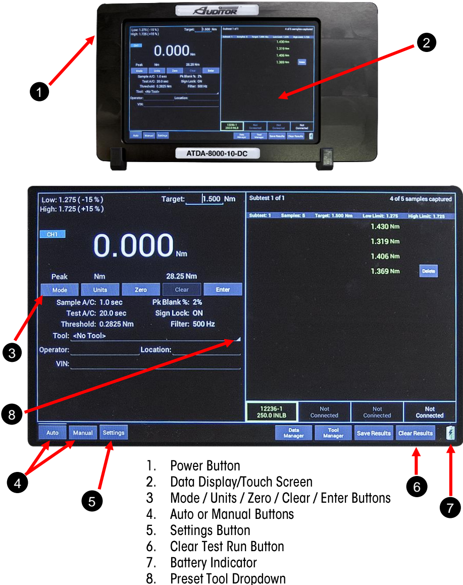
Figure 1: Main Screen
