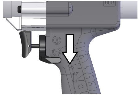
Set LEVER to L : Reverse
